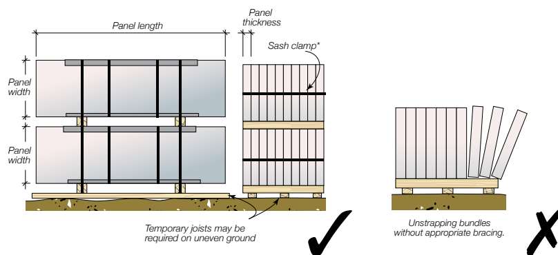
Figure 14.1 Stacking packs of STAAC WALL® panels
