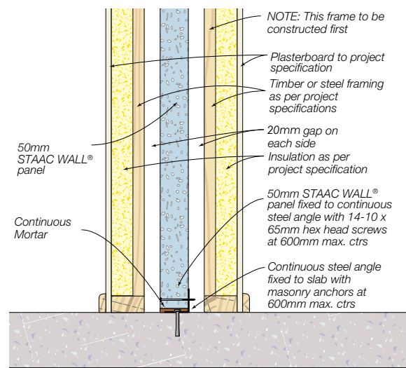
Figure 15.2.2 Base connection - Continuous steel angle
